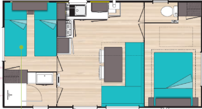
MH OPEHA 26m 2 - 2009 and 2012 5 persons- 2 bedrooms - 1 bathroom 1 toilet – paved terrace 9m 2
